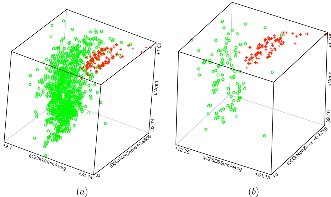
Figure 7: Scatter plots of the bleeding (denoted as red '+') and reference (green 'o') classes in the reduced feature subsets as selected by VSCH algorithm: a) training, b) test data vectors
