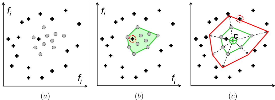
Figure 6: Illustration of convex hull method in 2D space ( k=2 )
