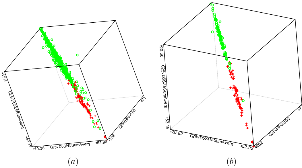
Figure 8: Scatter plots of the bleeding (denoted as red '+') and reference (green 'o') classes in the reduced feature subsets as selected by ANOVA algorithm: a) training, b) test data vectors
