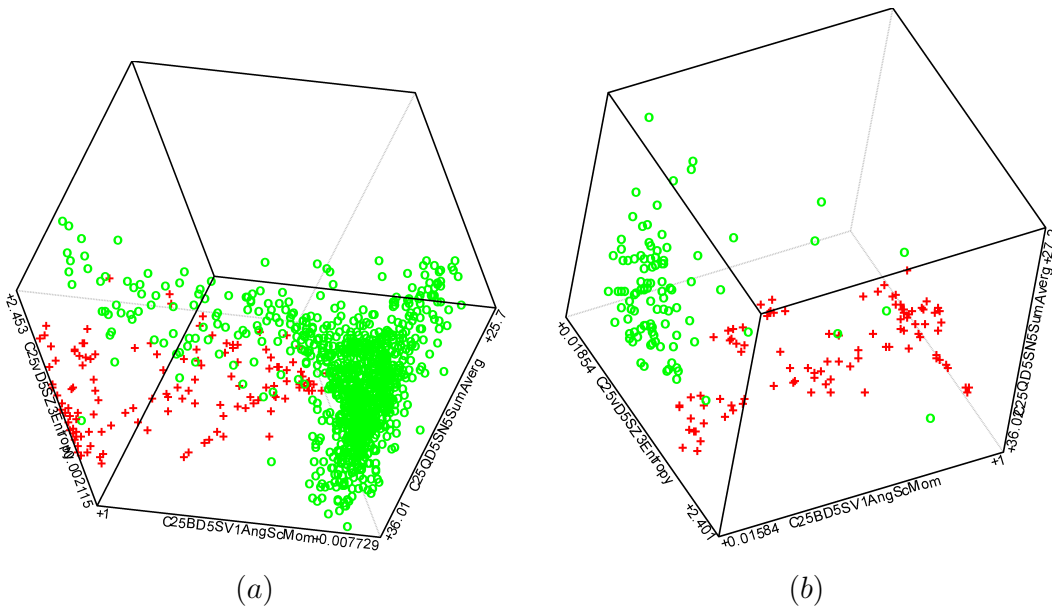
Figure 9: Scatter plots of the bleeding (denoted as red '+') and reference (green 'o') classes in the reduced feature subsets as selected by a-b) SVM/SFFS algorithm: a) training, b) test data vectors
